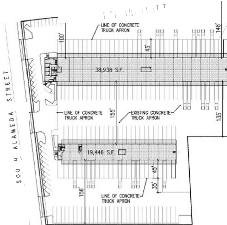
OVERALL PLAN - 550 SOUTH ALAMEDA STREET NOT TO SCALE. ALL DISTANCES ARE APPROXIMATE.
